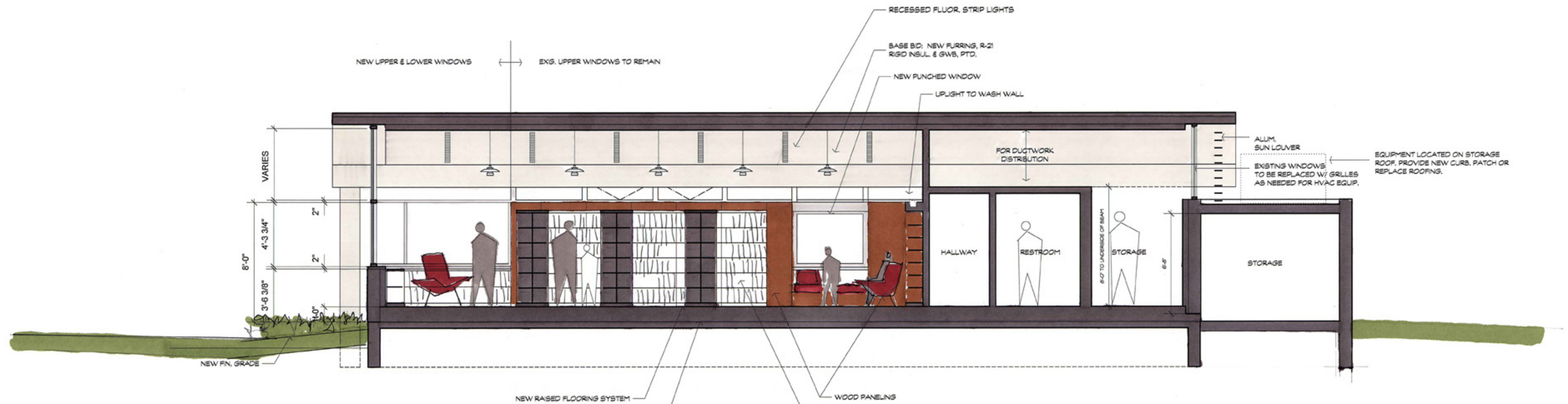
3 BUILDING SECTION DD2.4 Scale: 1/4" = 1'-0"
