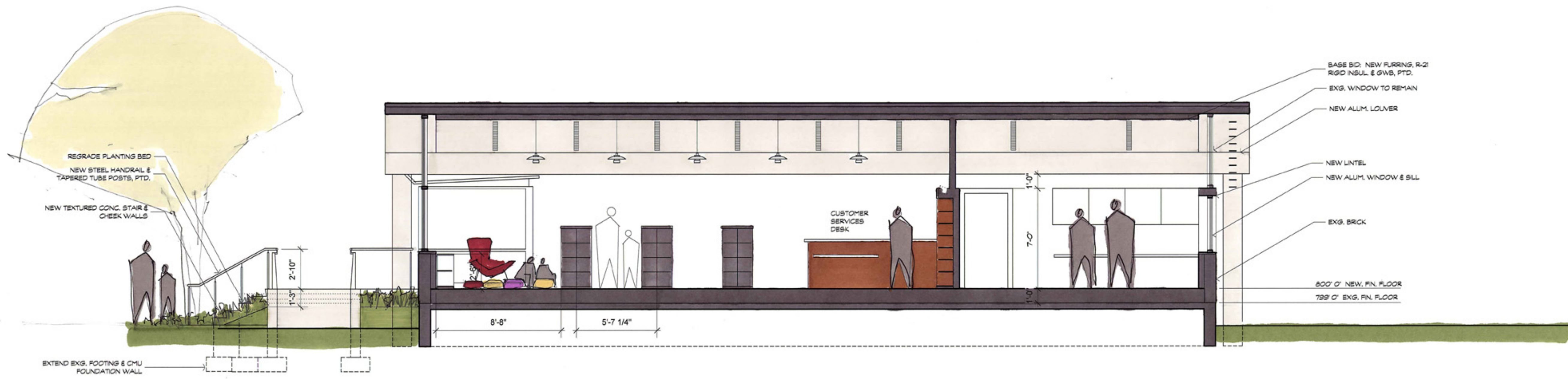
1 BUILDING SECTION DD2.4 Scale: 1/4" = 1'-0"
