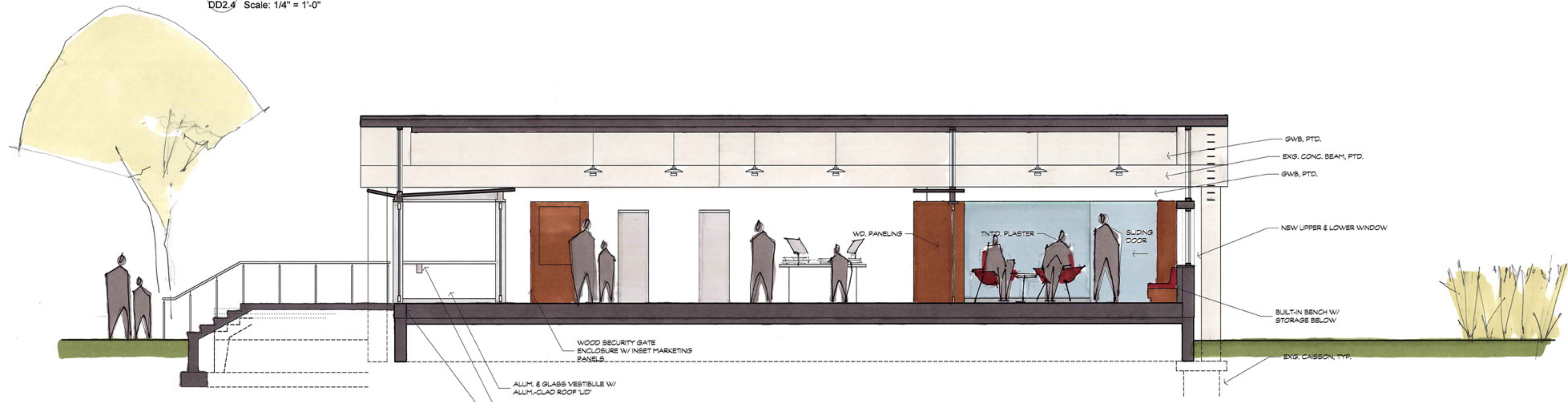
2 BUILDING SECTION DD2.4 Scale: 1/4" = 1'-0"
